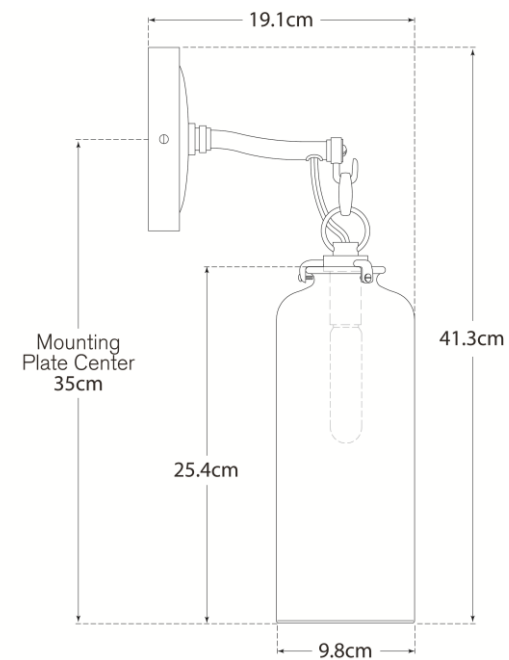
Front View Mounting Plate
